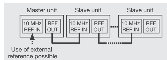
Connection method 2 (up to 4 units)
